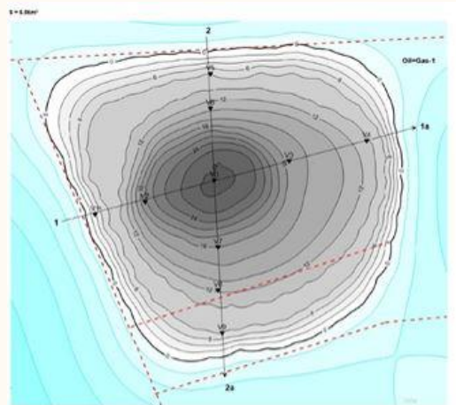
Fault zones are shown in red. Black lines indicate relative signal response levels. An in-depth scan was made over two sections of the deposit 1 - 1a and 2 - 2a at points V0 - V4 and V5 - V9, respectively. The following figure shows an example of a deep section of the oil horizon at points V0 - V4.
